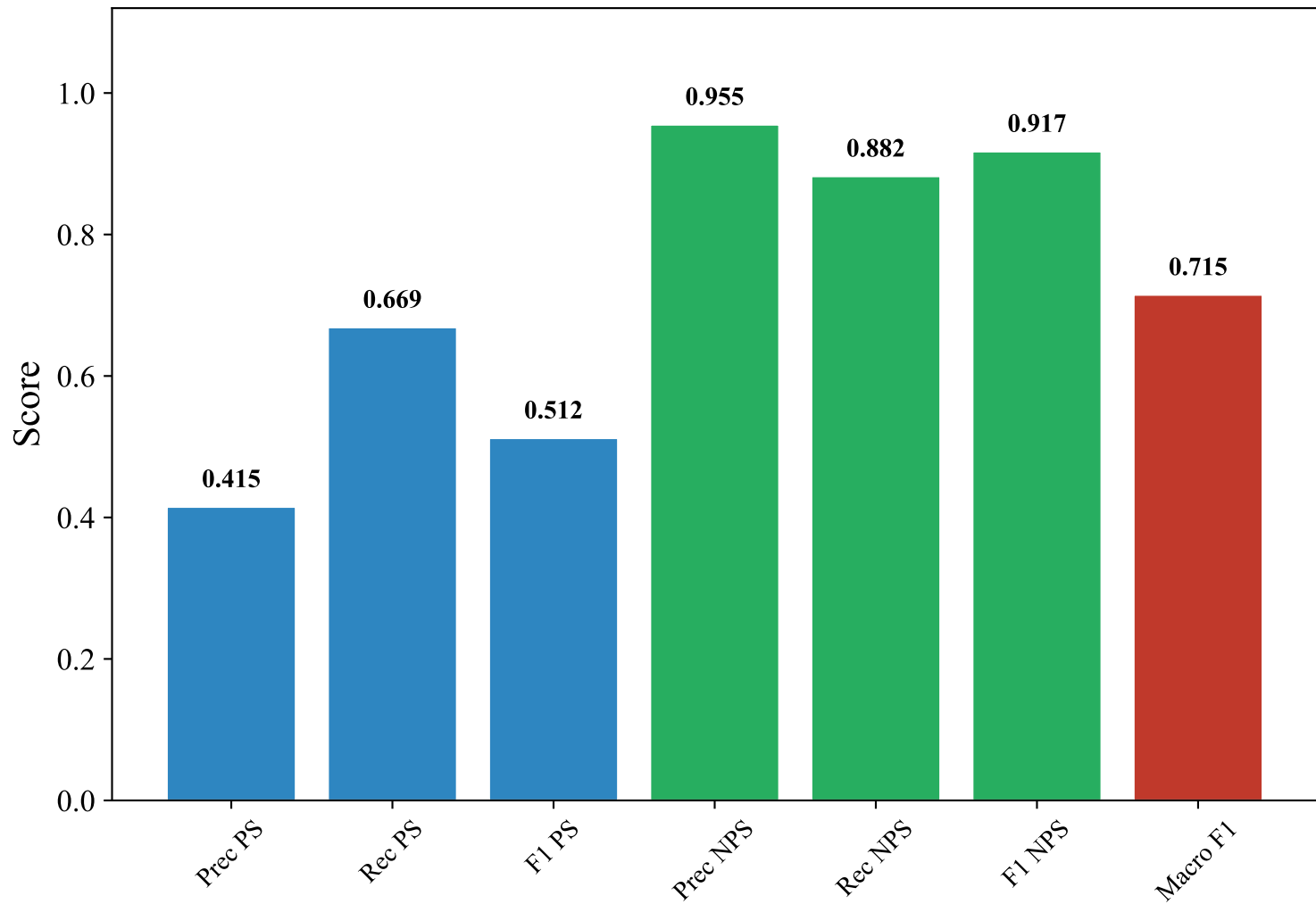
Classification Metrics — GERMAN_MANUAL (intfloat/multilingual-e5-large-instruct, Voting_Ensemble)
