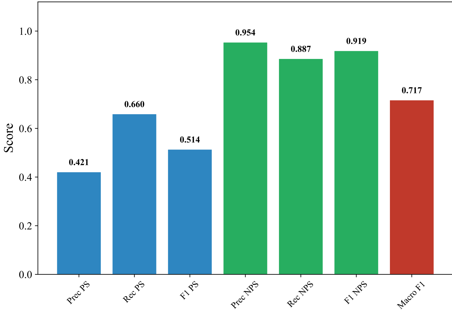
Classification Metrics — GERMAN_MANUAL (intfloat/multilingual-e5-large-instruct, XGBoost_Optimized)
