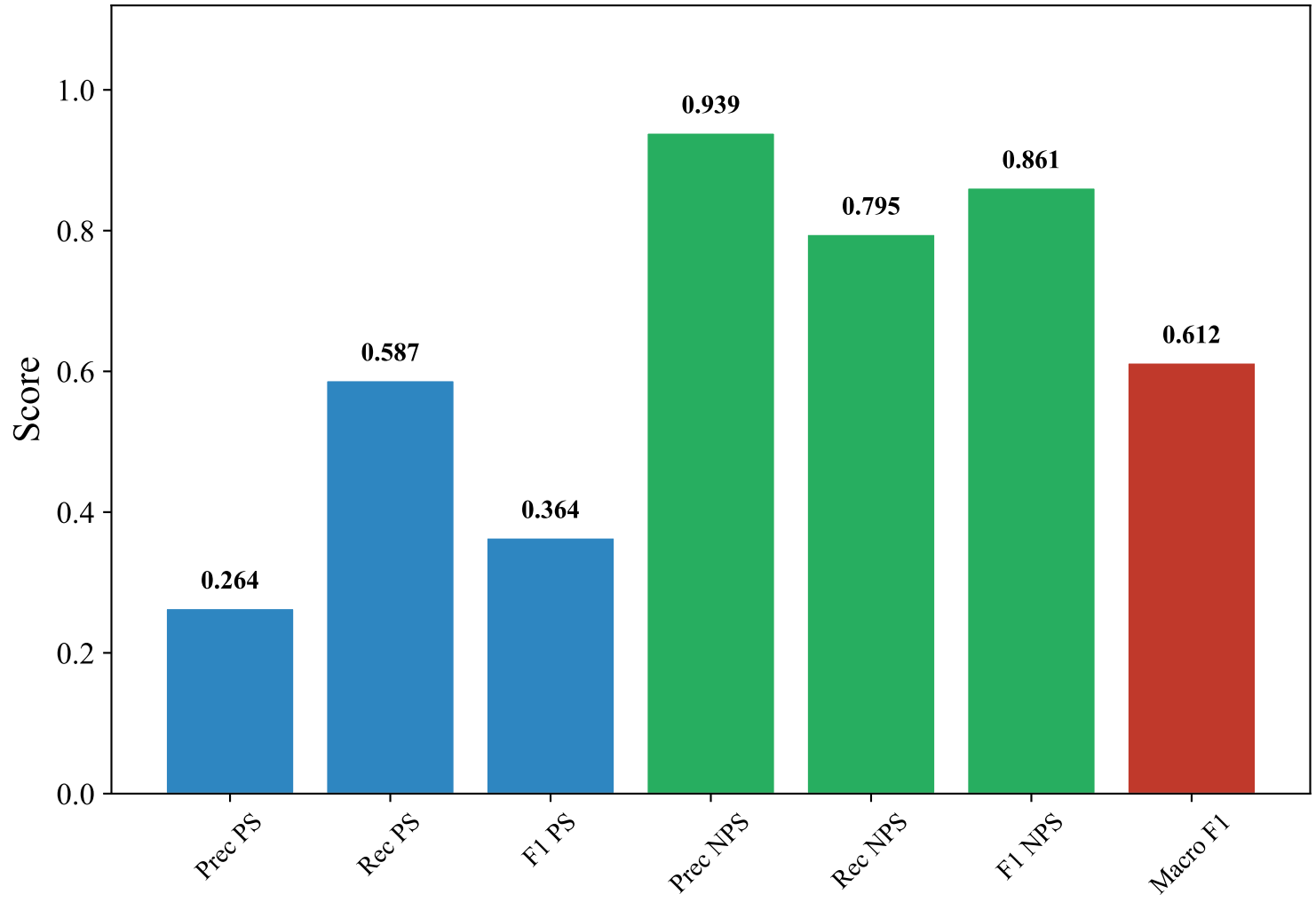
Classification Metrics — GERMAN_MANUAL (paraphrase-multilingual-MiniLM-L12-v2, LightGBM)
