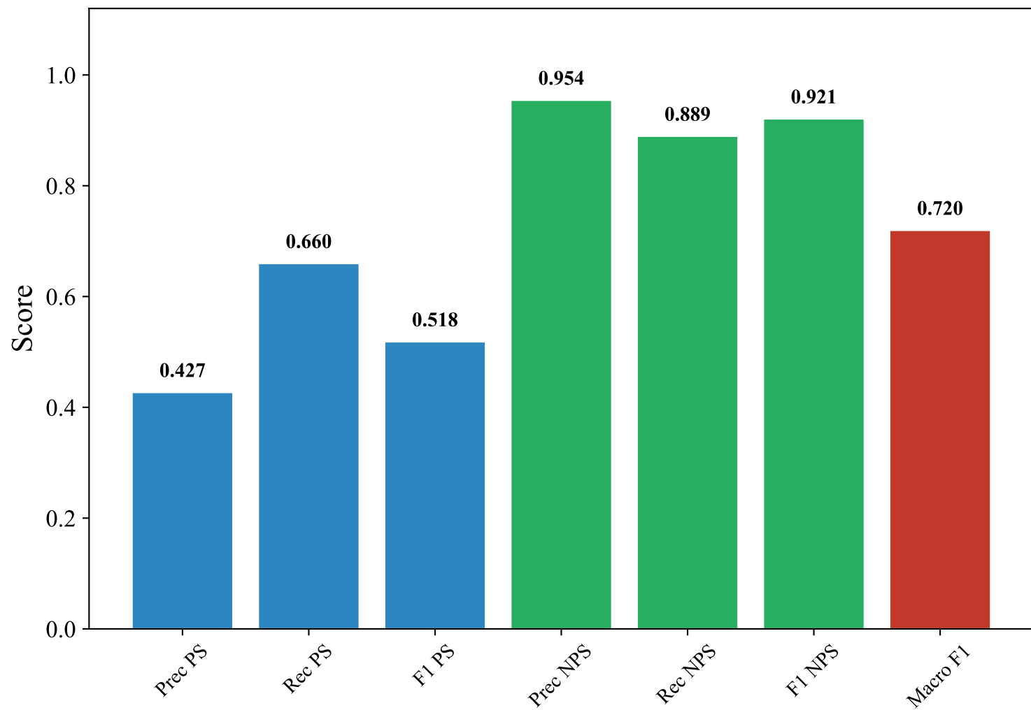
Classification Metrics — GERMAN_MANUAL (snowflake-arctic-embed-l-v2.0, LightGBM_Optimized)
