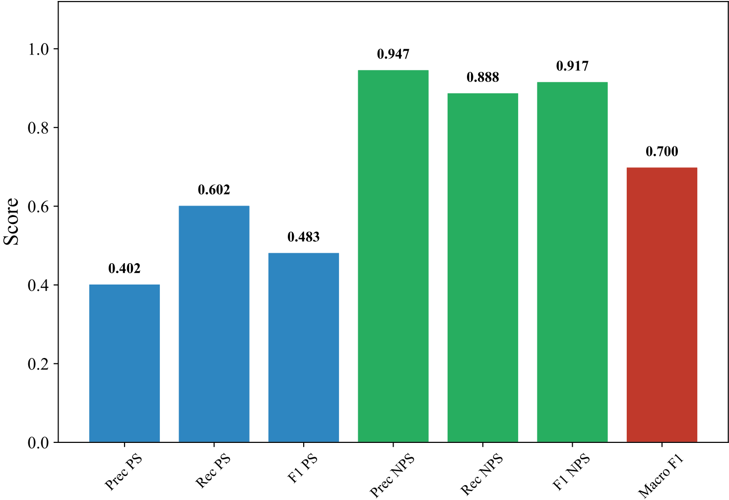
Classification Metrics — GERMAN_MANUAL (upskyy/bge-m3-korean, LightGBM_Optimized)
