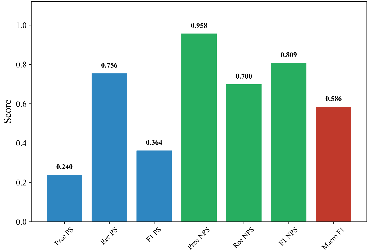
Classification Metrics — GERMAN_MANUAL (upskyy/bge-m3-korean, Random_Forest)
