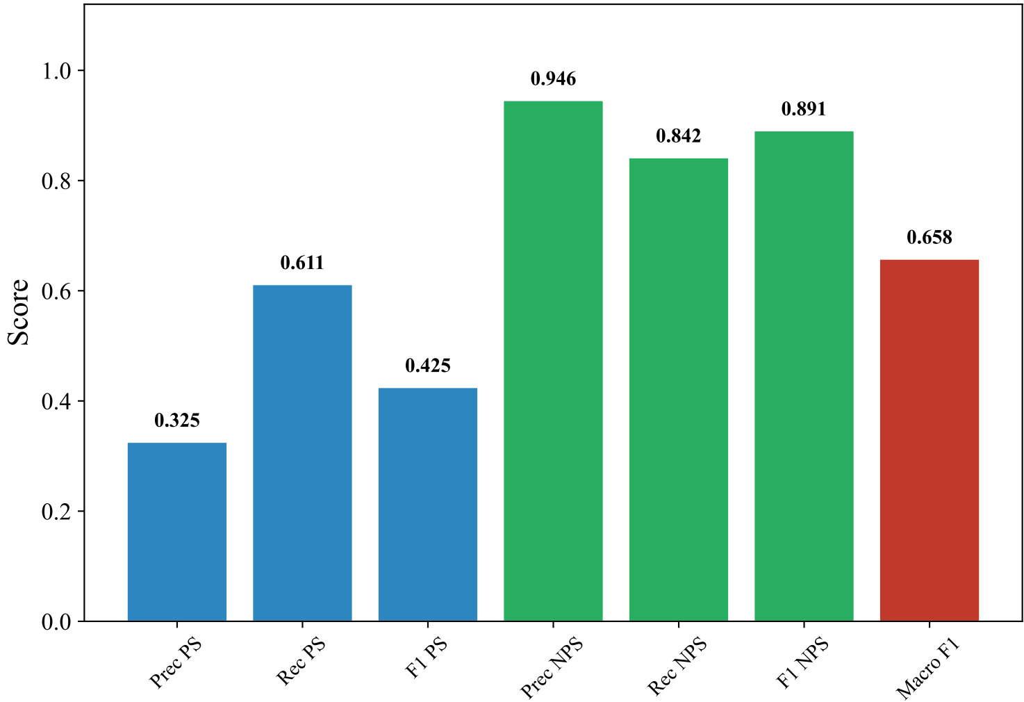
Classification Metrics — GERMAN_MANUAL (upskyy/bge-m3-korean, SVM)
