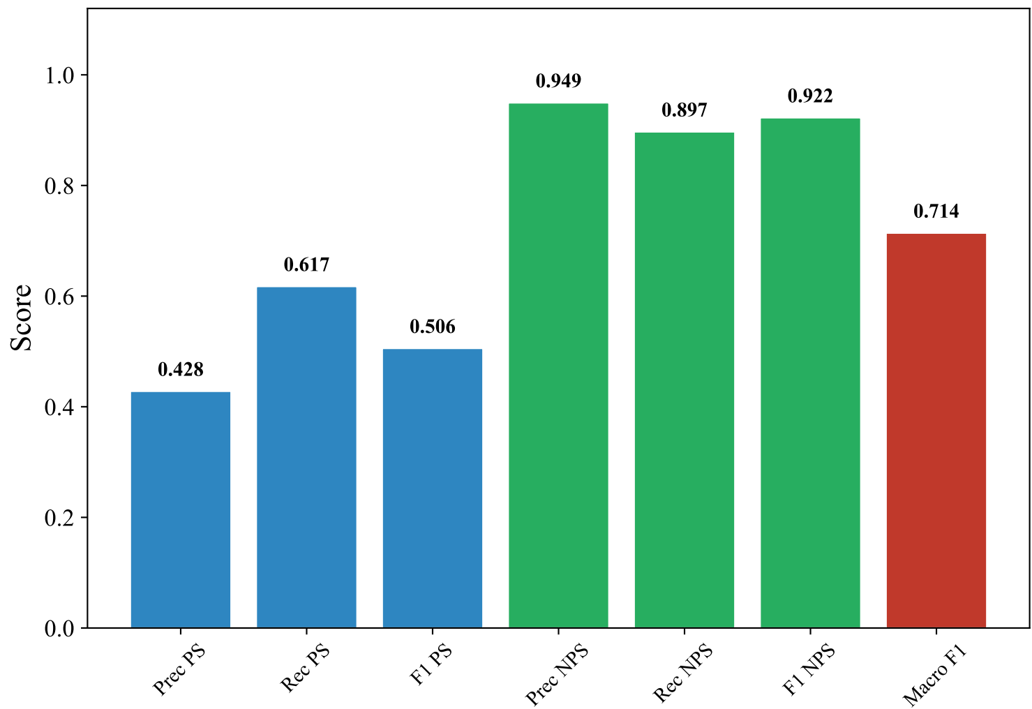
Classification Metrics — GERMAN_MANUAL (upskyy/bge-m3-korean, XGBoost)
