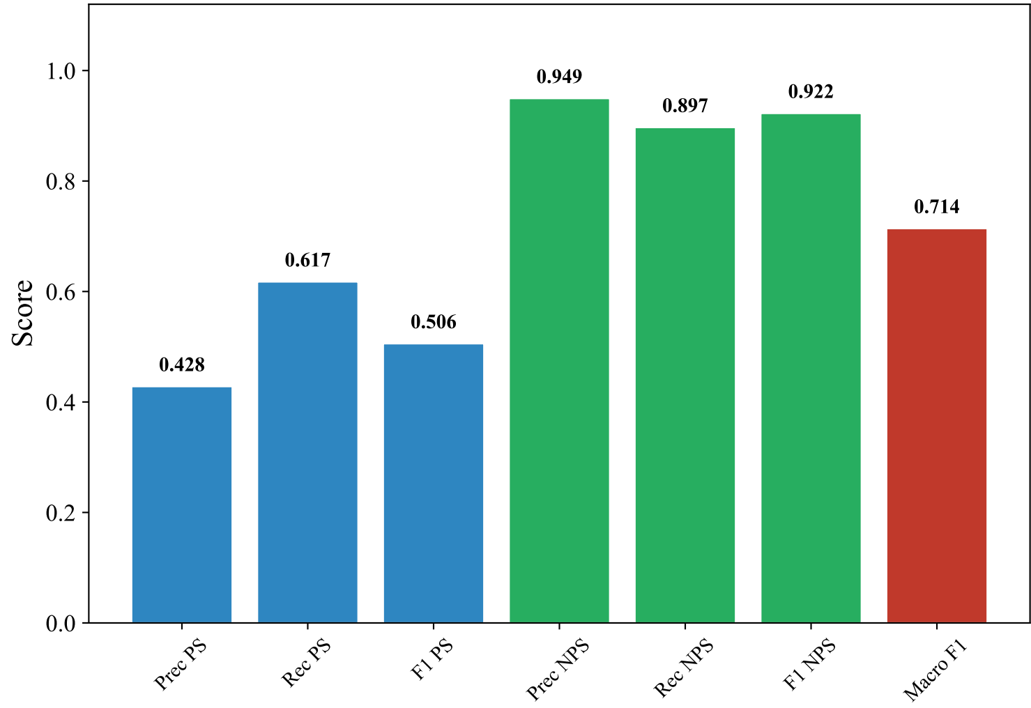
Classification Metrics — GERMAN_MANUAL (upskyy/bge-m3-korean, XGBoost_Optimized)
