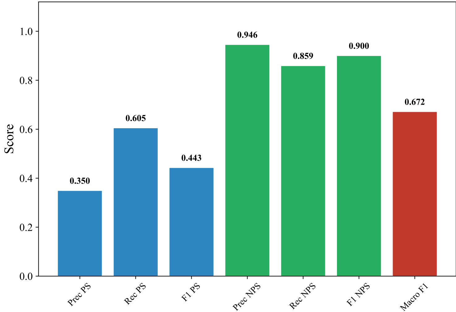
Classification Metrics — GERMAN_MANUAL (xlm-roberta-base, LightGBM_Optimized)
