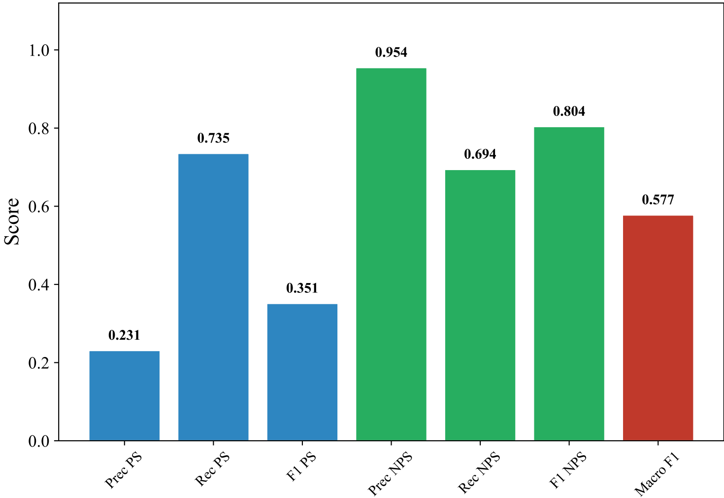
Classification Metrics — GERMAN_MANUAL (xlm-roberta-base, Random_Forest)
