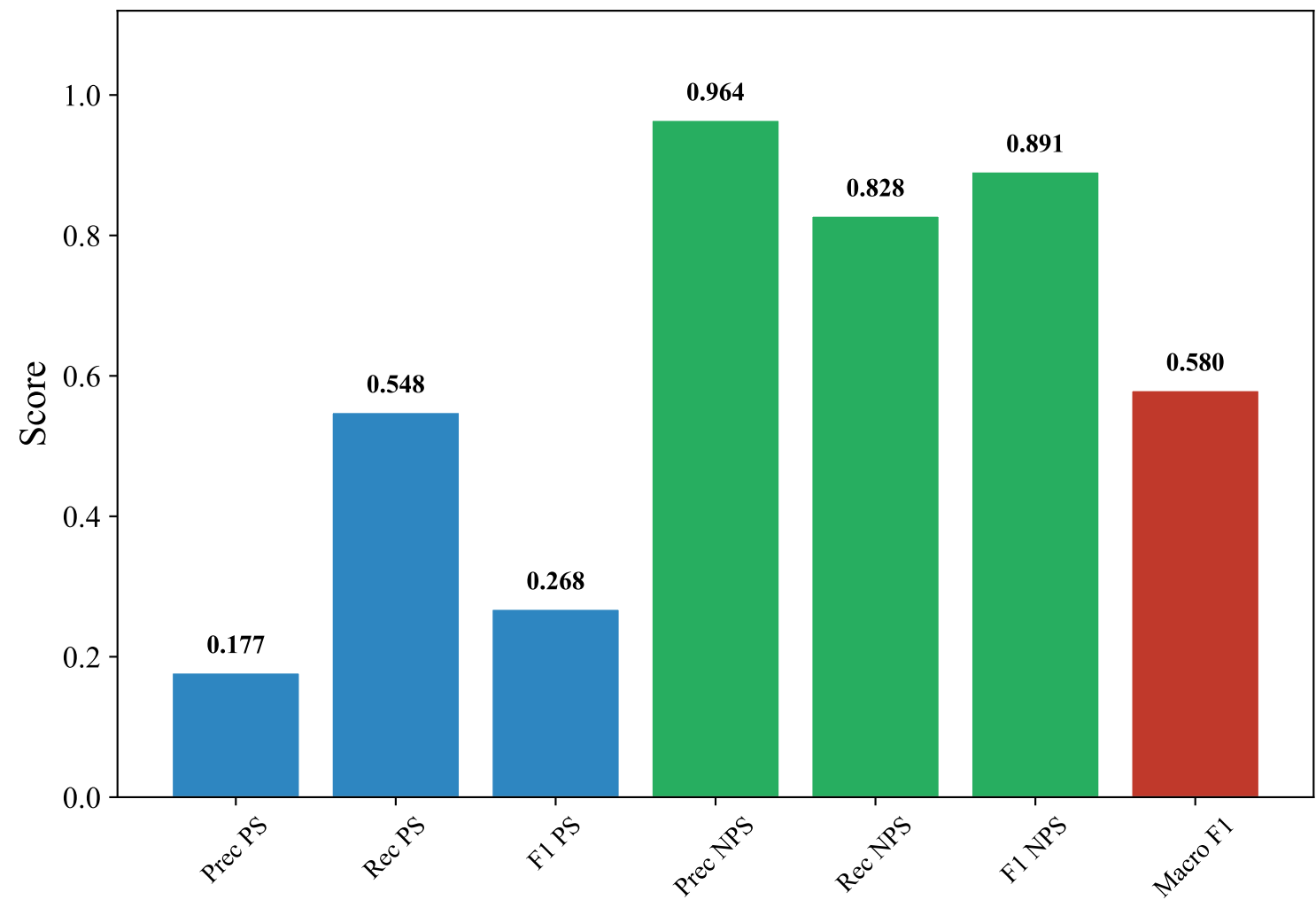
Classification Metrics — SWEDISH_MANUAL (bert-base-multilingual-uncased, SVM)
