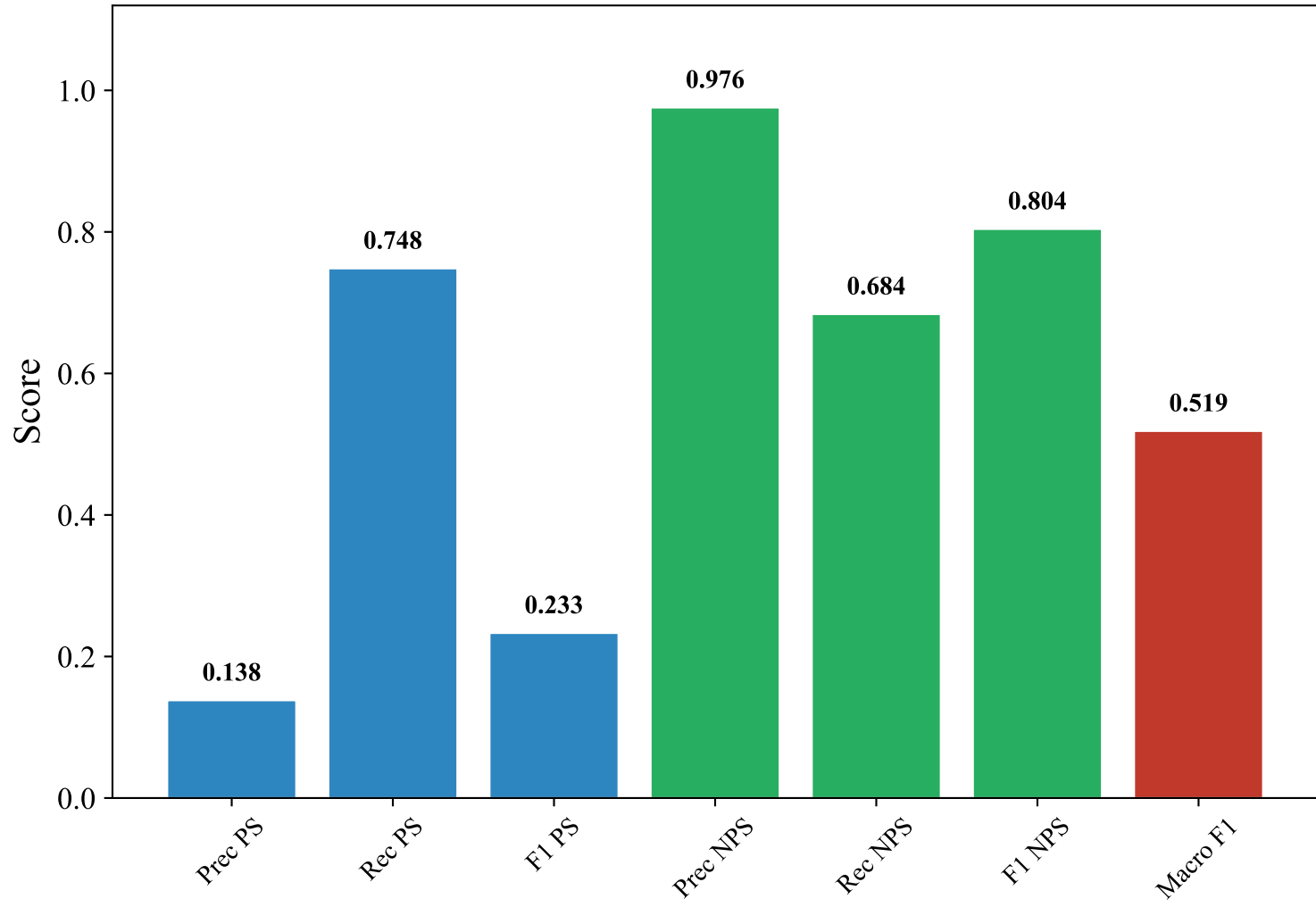
Classification Metrics — SWEDISH_MANUAL (efederici/e5-base-multilingual-4096, Random_Forest)
