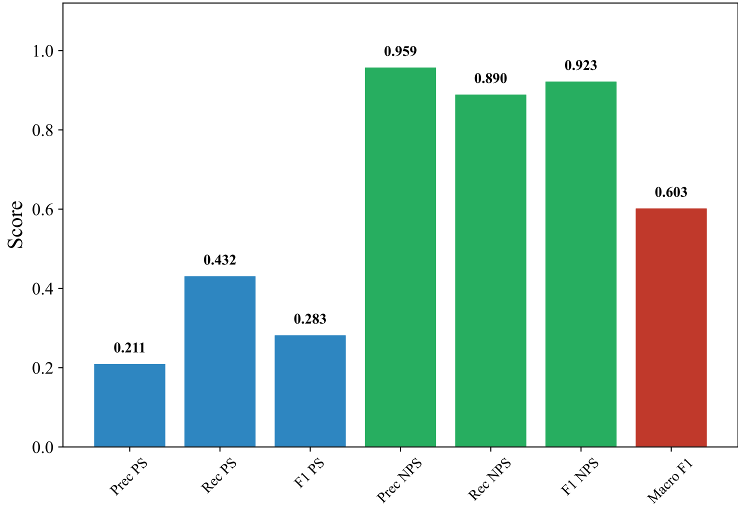
Classification Metrics — SWEDISH_MANUAL (efederici/e5-base-multilingual-4096, Voting_Ensemble)
