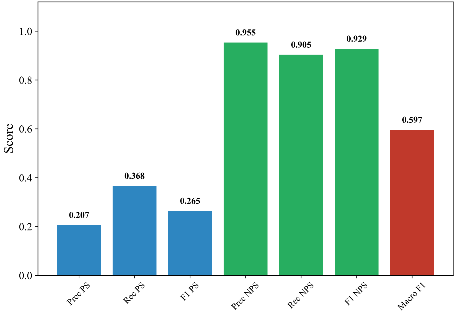
Classification Metrics — SWEDISH_MANUAL (efederici/e5-base-multilingual-4096, XGBoost)
