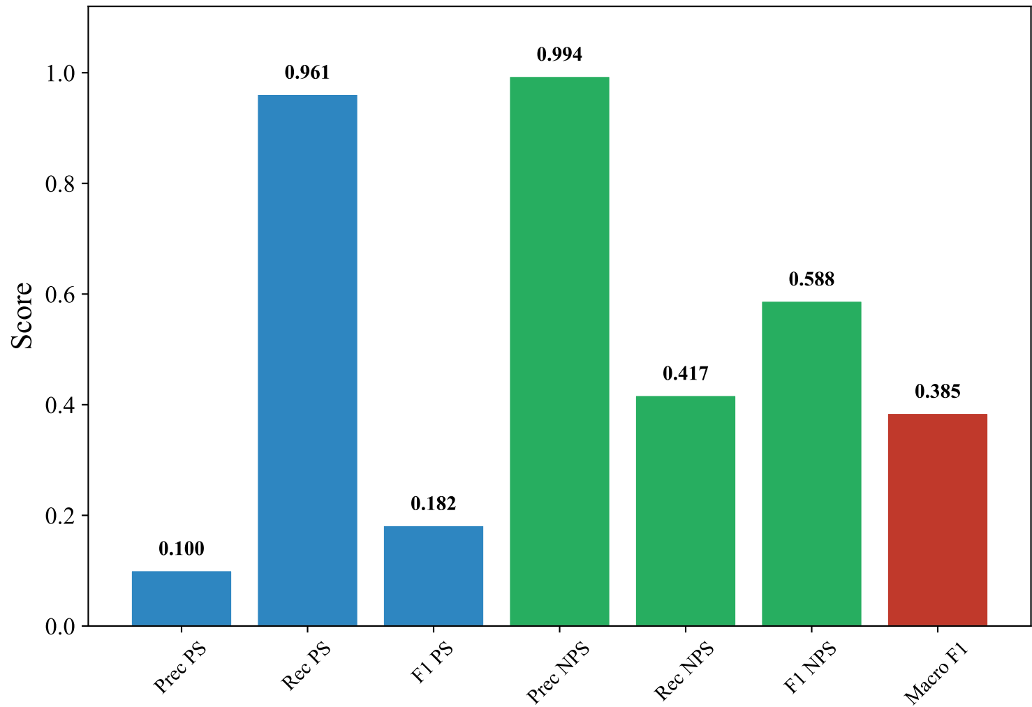
Classification Metrics — SWEDISH_MANUAL (intfloat/multilingual-e5-large-instruct, Random_Forest_Optimized)
