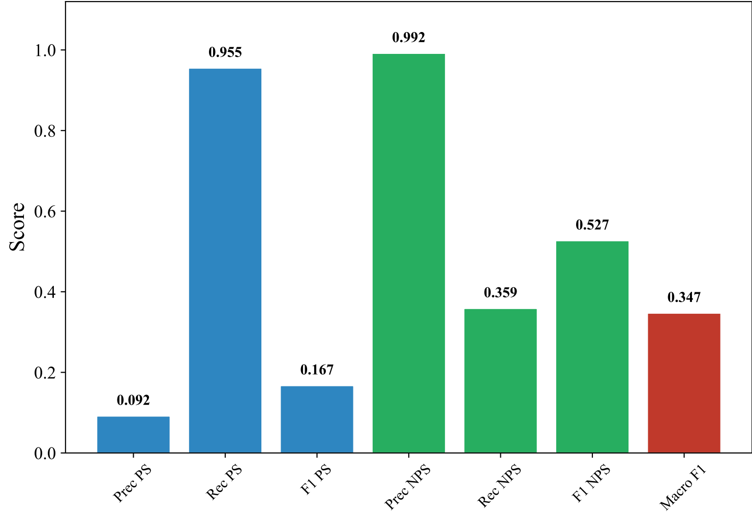
Classification Metrics — SWEDISH_MANUAL (paraphrase-multilingual-MiniLM-L12-v2, Random_Forest_Optimized)
