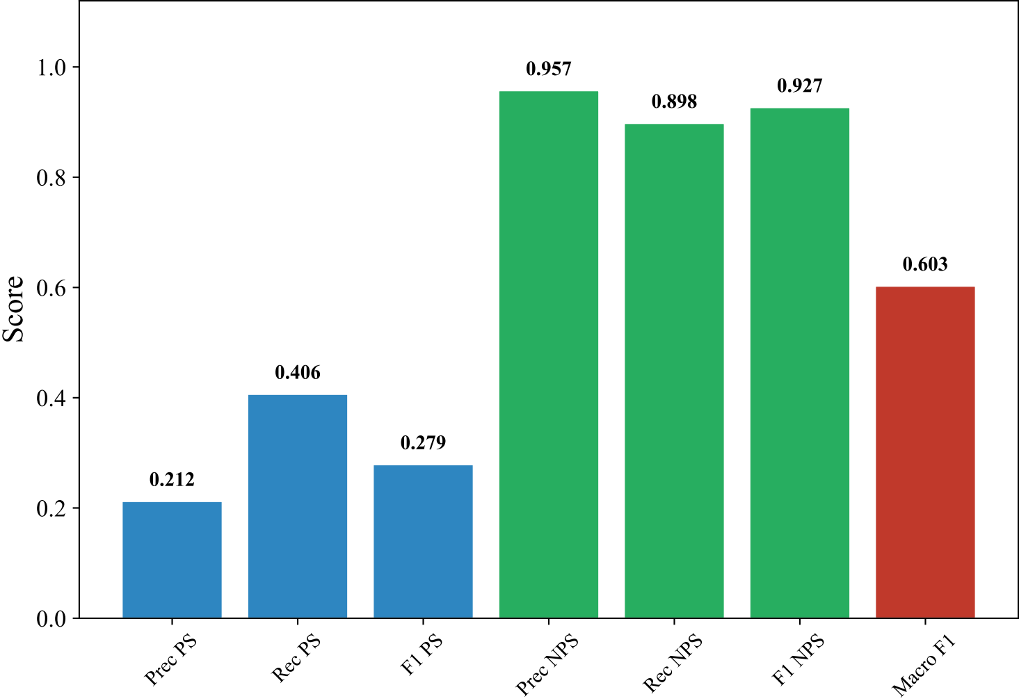
Classification Metrics — SWEDISH_MANUAL (paraphrase-multilingual-mpnet-base-v2, LightGBM_Optimized)
