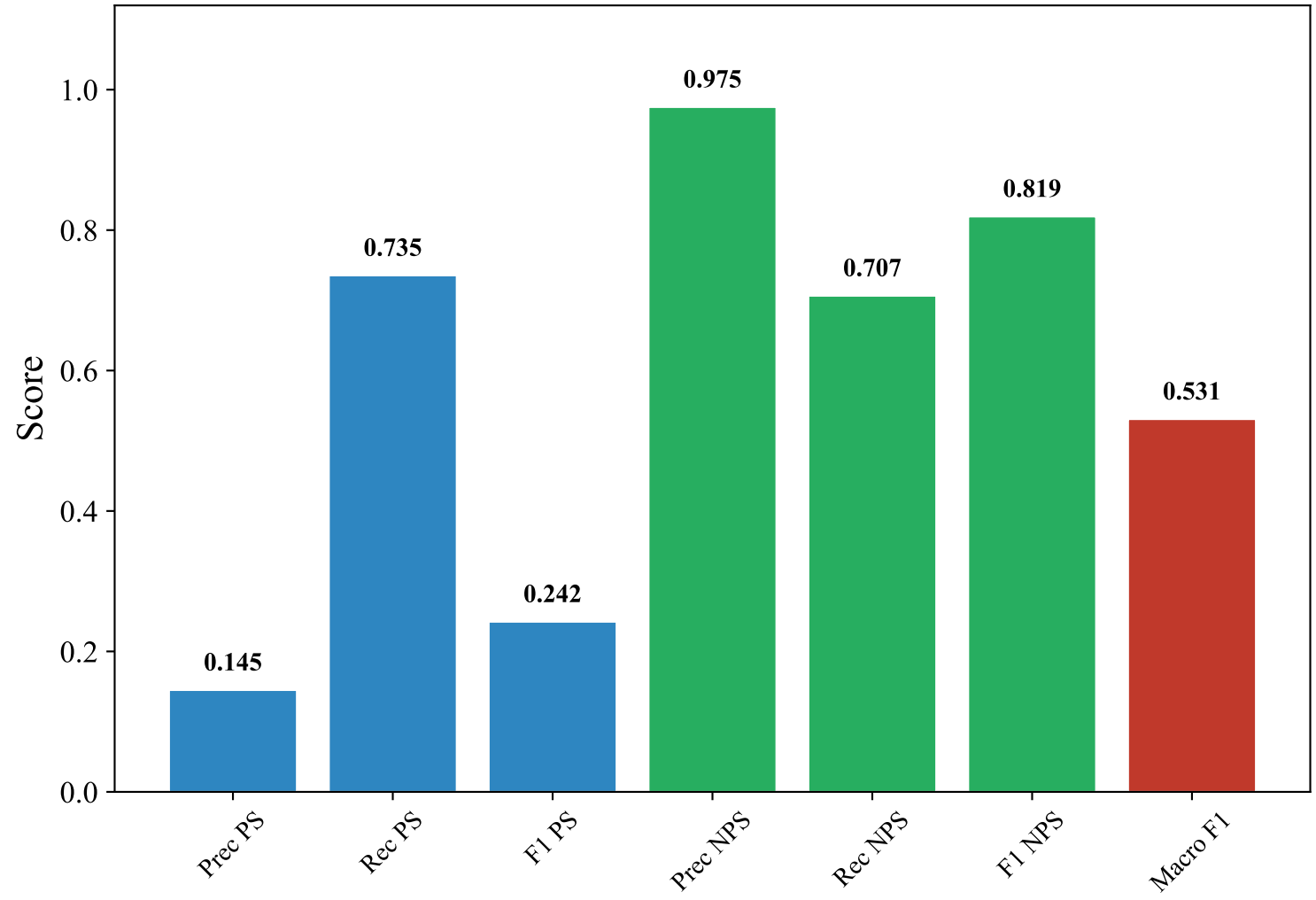
Classification Metrics — SWEDISH_MANUAL (snowflake-arctic-embed-l-v2.0, Random_Forest)
