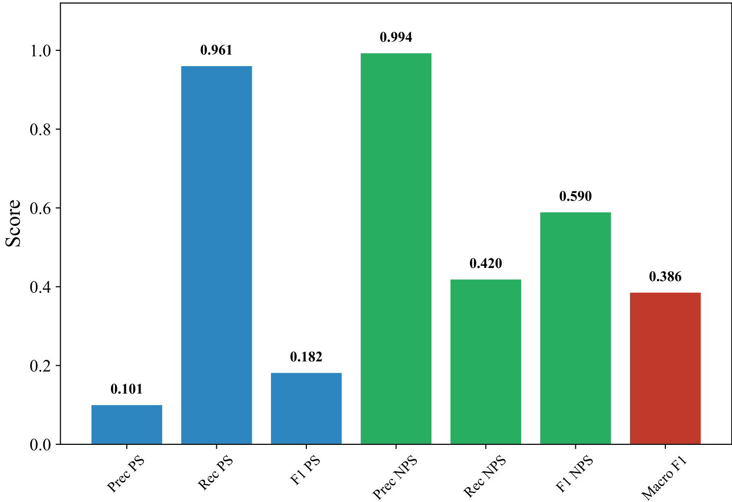
Classification Metrics — SWEDISH_MANUAL (snowflake-arctic-embed-l-v2.0, Random_Forest_Optimized)
