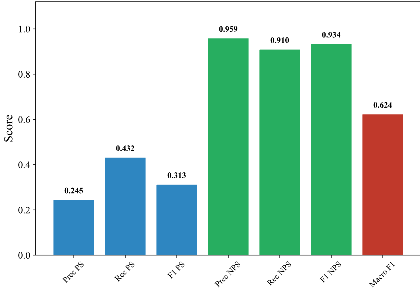
Classification Metrics — SWEDISH_MANUAL (snowflake-arctic-embed-l-v2.0, XGBoost_Optimized)
