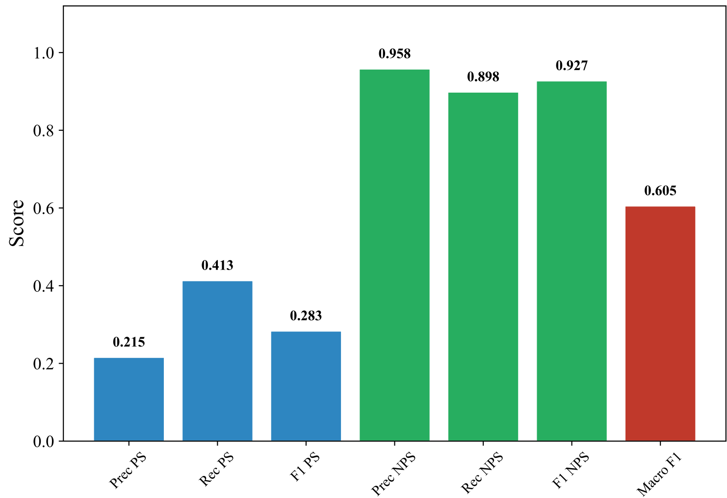
Classification Metrics — SWEDISH_MANUAL (upskyy/bge-m3-korean, LightGBM)
