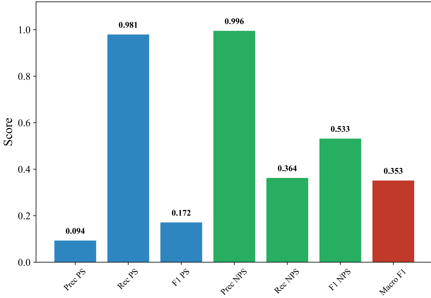
Classification Metrics — SWEDISH_MANUAL (upskyy/bge-m3-korean, Random_Forest_Optimized)
