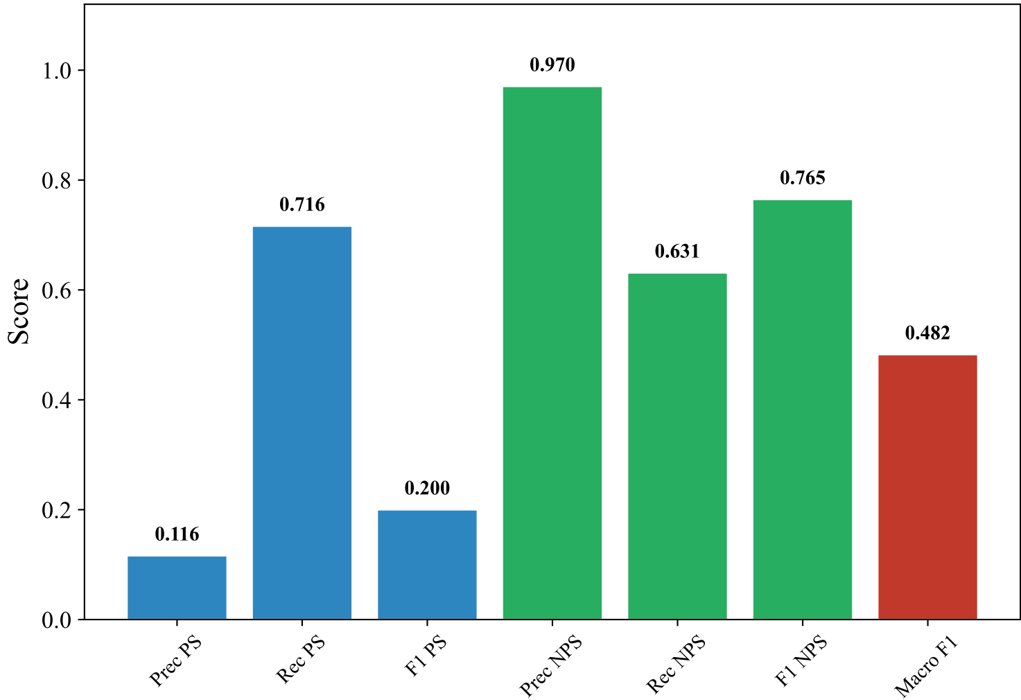
Classification Metrics — SWEDISH_MANUAL (xlm-roberta-base, Random_Forest)
