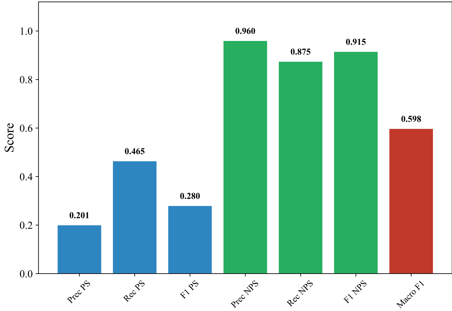
Classification Metrics — SWEDISH_MANUAL (xlm-roberta-base, Voting_Ensemble)
