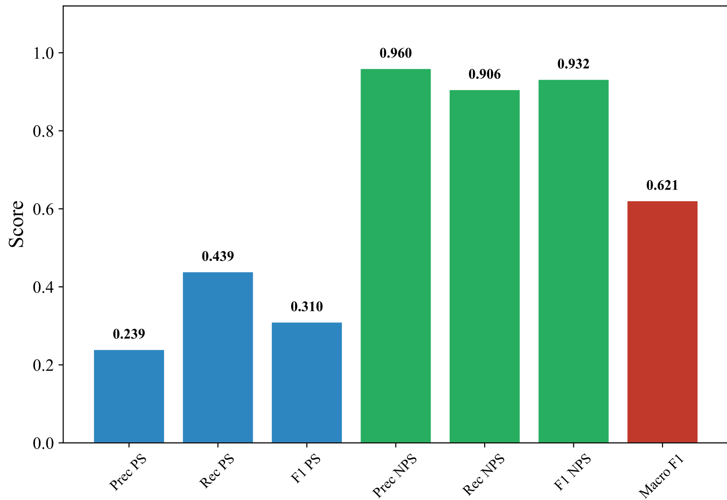
Classification Metrics — SWEDISH_MANUAL (xlm-roberta-base, XGBoost_Optimized)
