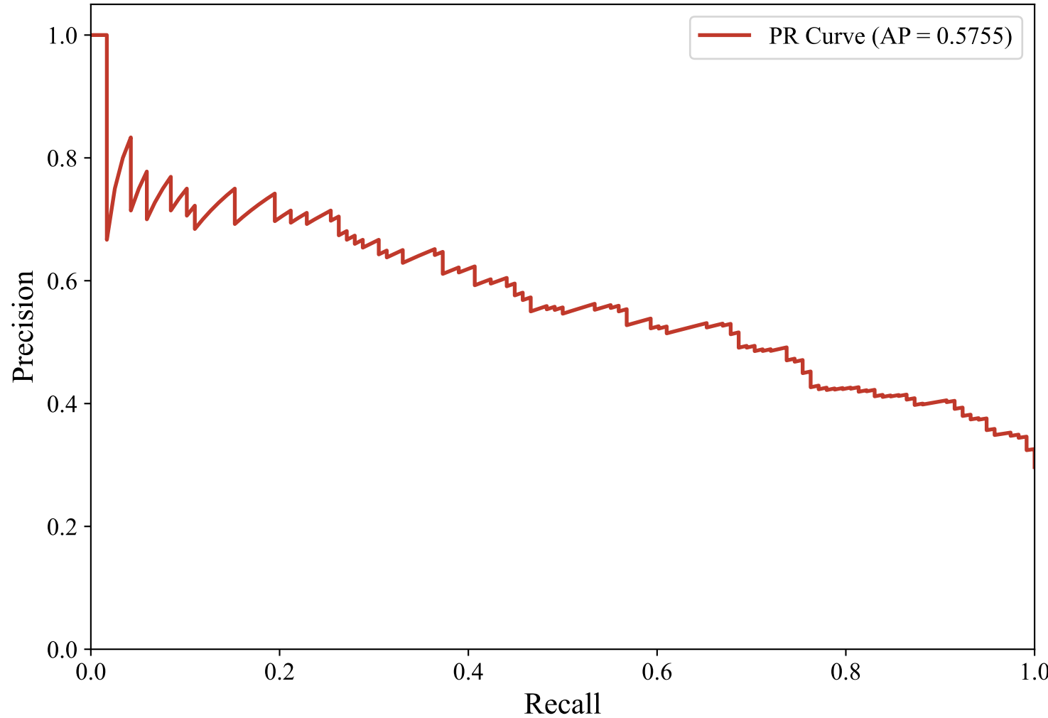
Precision-Recall Curve — DUTCH_MANUAL (bert-base-multilingual-uncased, LightGBM_Optimized)
