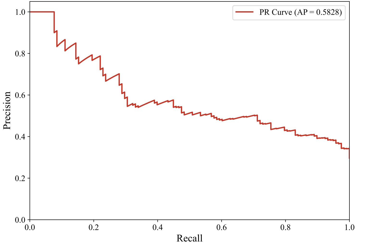
Precision-Recall Curve — DUTCH_MANUAL (bert-base-multilingual-uncased, XGBoost_Optimized)
