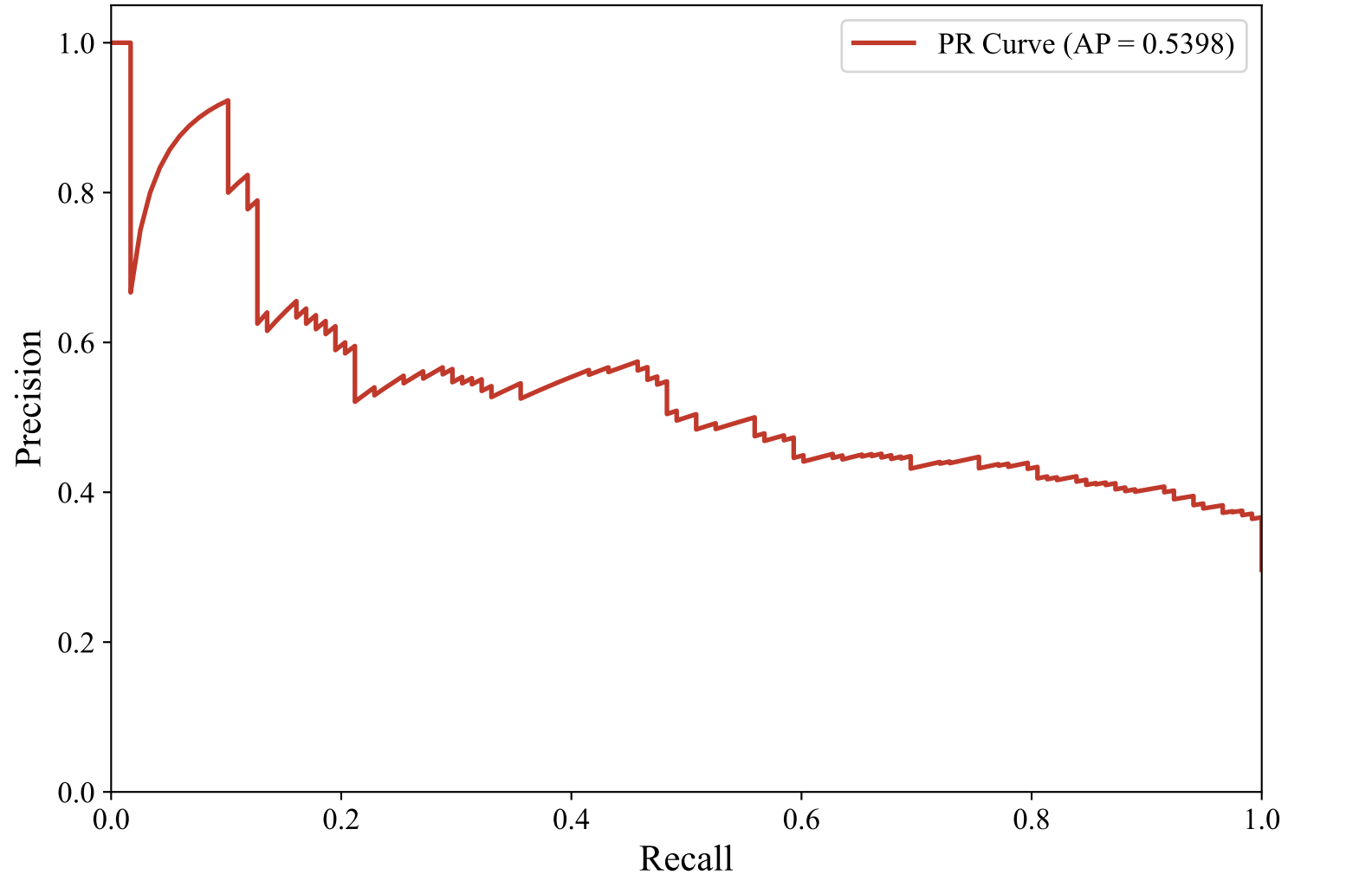
Precision-Recall Curve — DUTCH_MANUAL (efederici/e5-base-multilingual-4096, Random_Forest)
