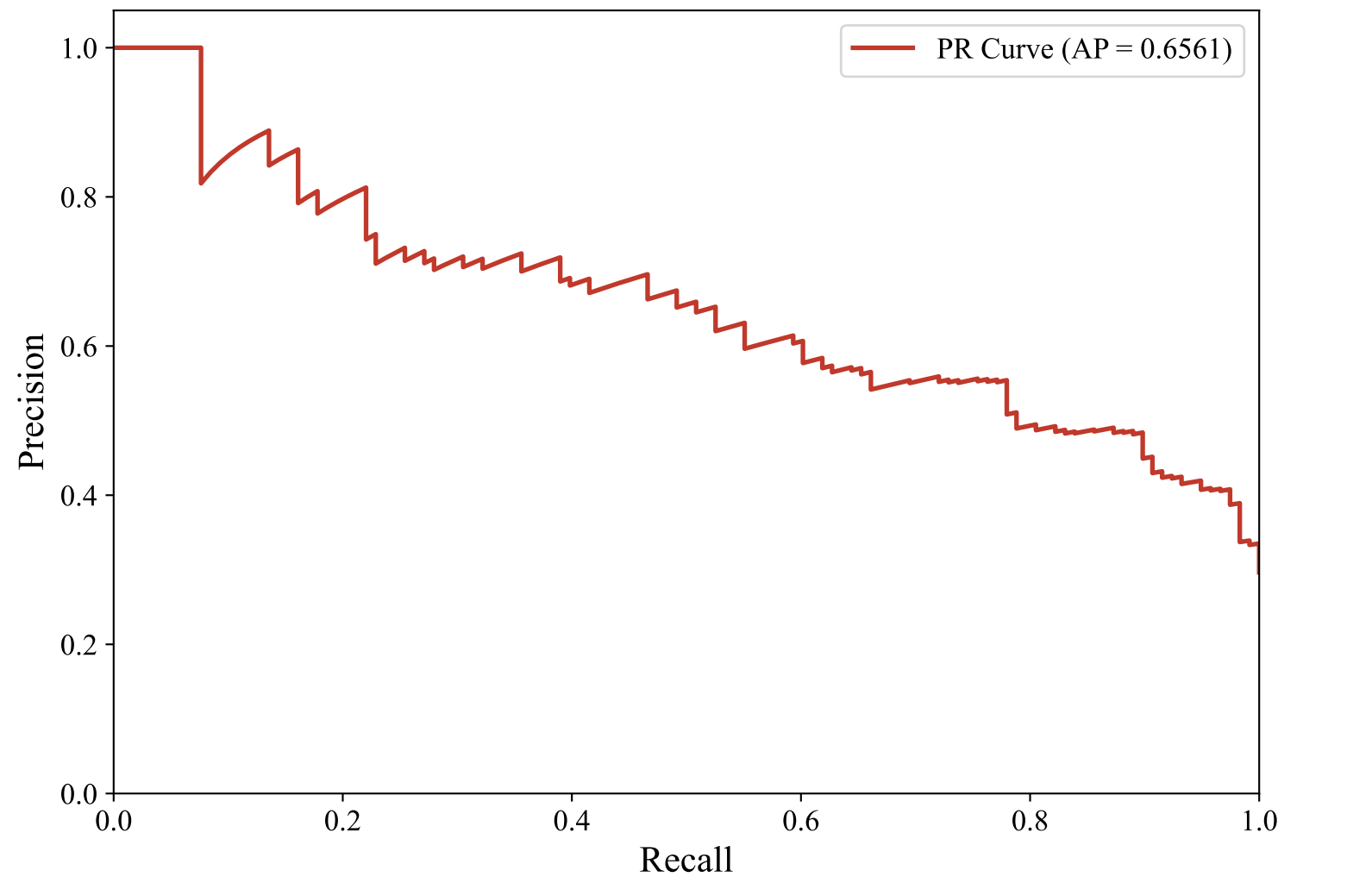
Precision-Recall Curve — DUTCH_MANUAL (efederici/e5-base-multilingual-4096, XGBoost_Optimized)
