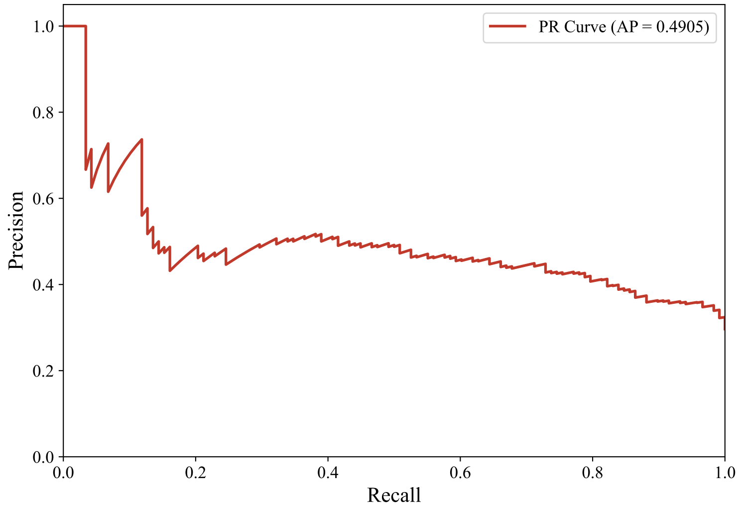
Precision-Recall Curve — DUTCH_MANUAL (paraphrase-multilingual-MiniLM-L12-v2, Random_Forest_Optimized)
