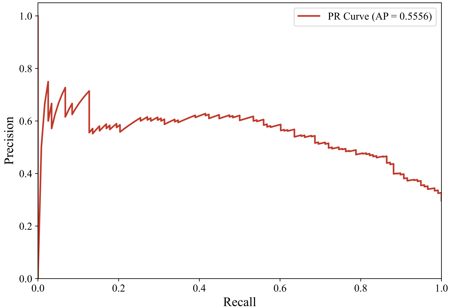
Precision-Recall Curve — DUTCH_MANUAL (paraphrase-multilingual-MiniLM-L12-v2, Voting_Ensemble)
