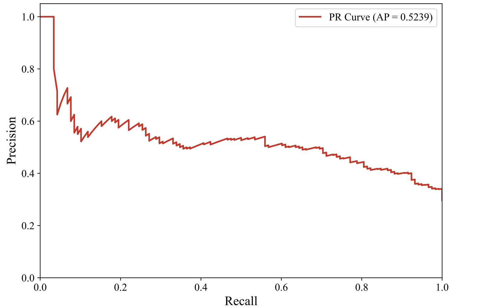
Precision-Recall Curve — DUTCH_MANUAL (paraphrase-multilingual-mpnet-base-v2, Random_Forest)
