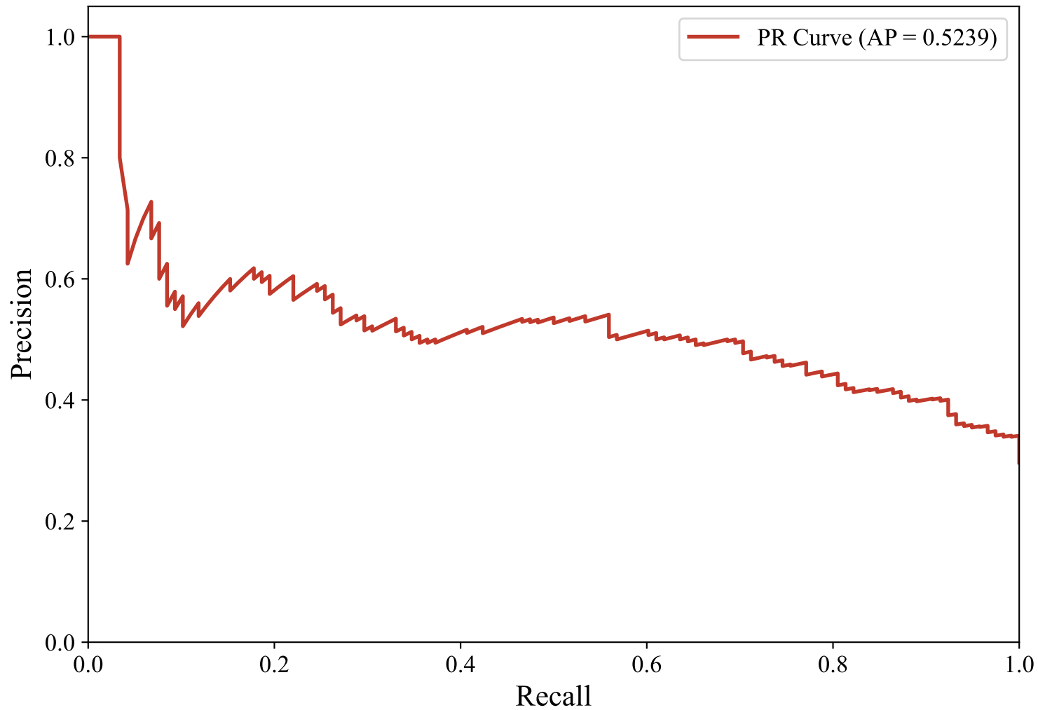
Precision-Recall Curve — DUTCH_MANUAL (paraphrase-multilingual-mpnet-base-v2, Random_Forest_Optimized)
