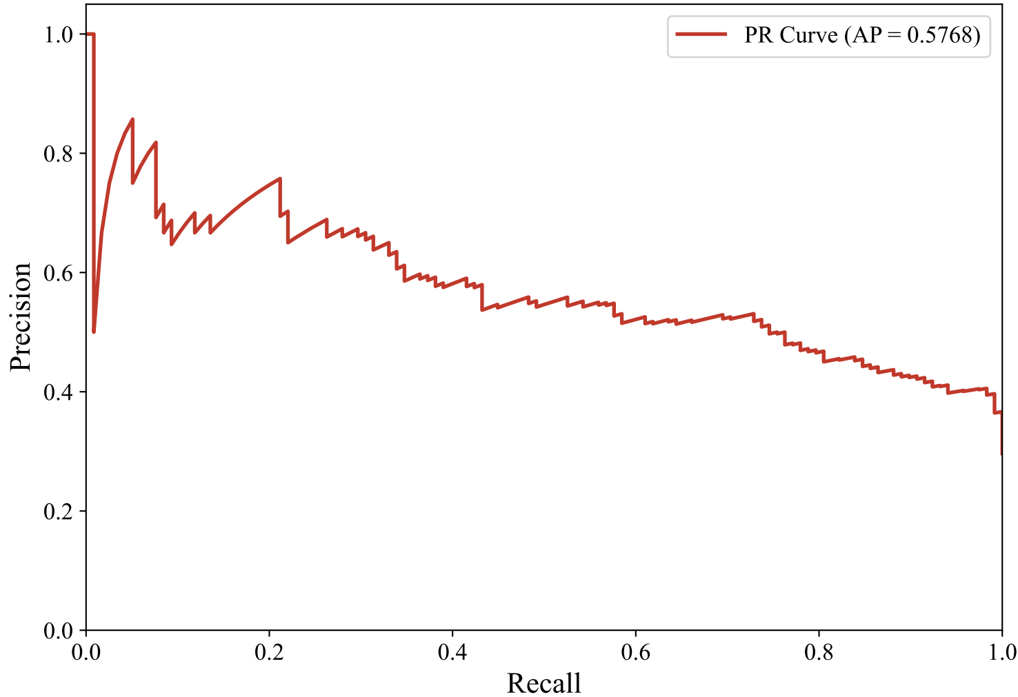
Precision-Recall Curve — DUTCH_MANUAL (snowflake-arctic-embed-l-v2.0, Random_Forest)
