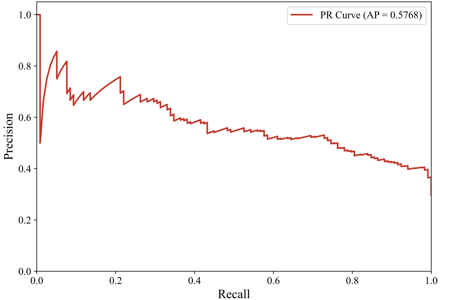
Precision-Recall Curve — DUTCH_MANUAL (snowflake-arctic-embed-l-v2.0, Random_Forest_Optimized)
