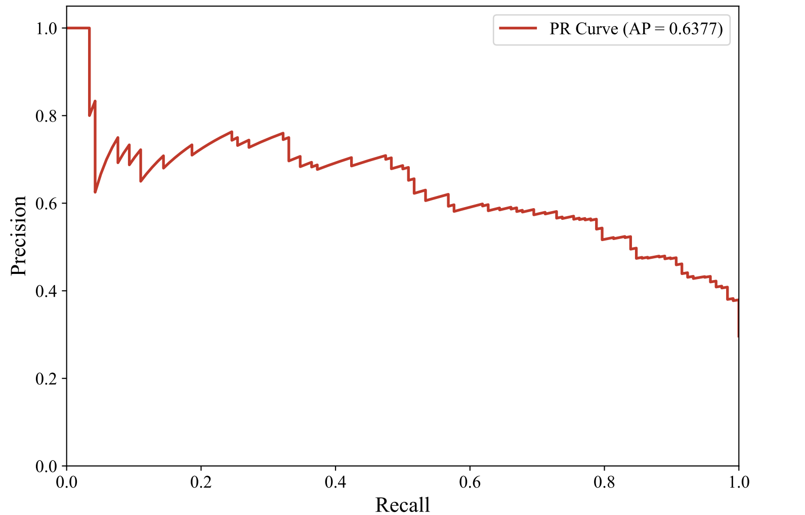
Precision-Recall Curve — DUTCH_MANUAL (snowflake-arctic-embed-l-v2.0, Voting_Ensemble)
