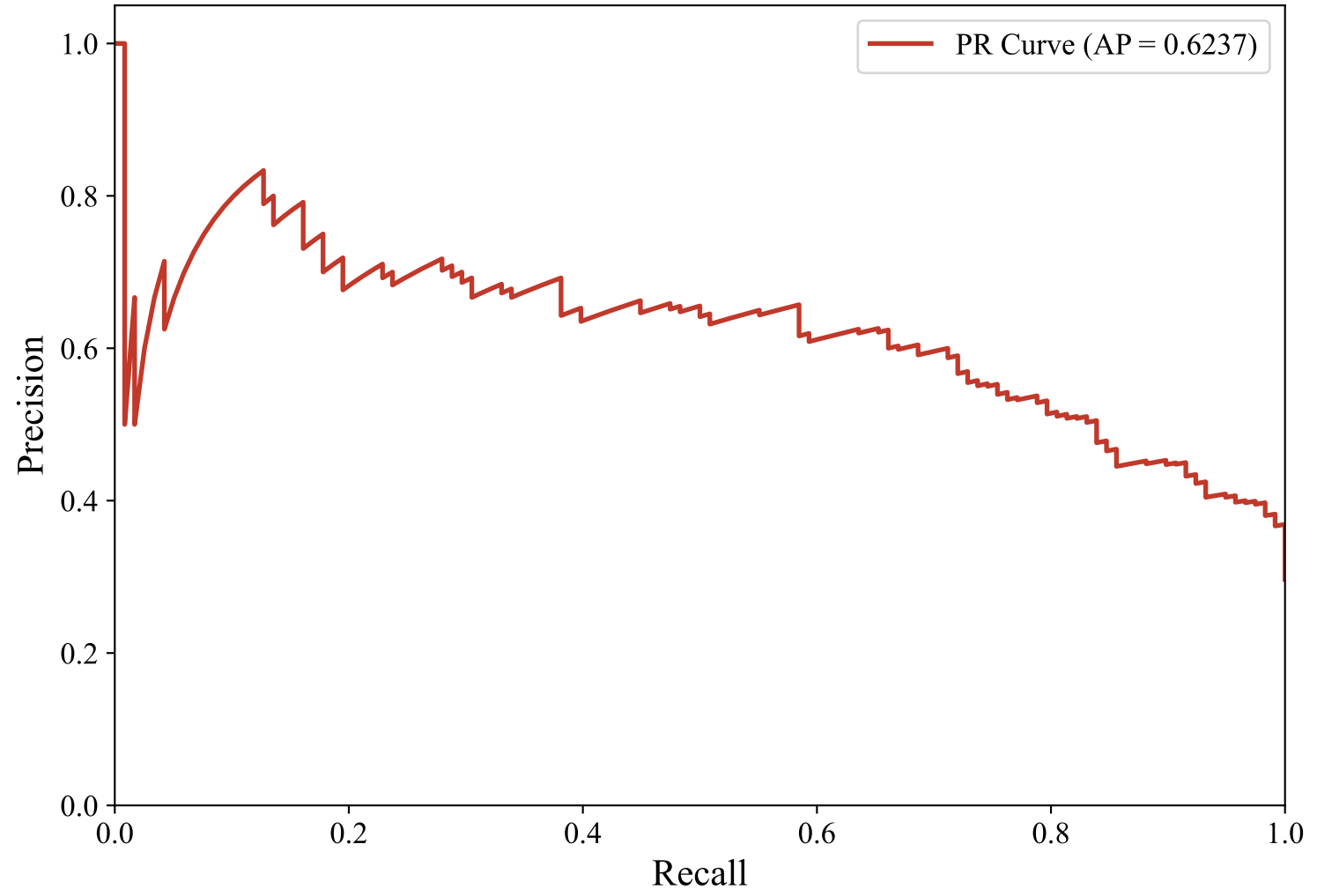
Precision-Recall Curve — DUTCH_MANUAL (snowflake-arctic-embed-l-v2.0, XGBoost)
