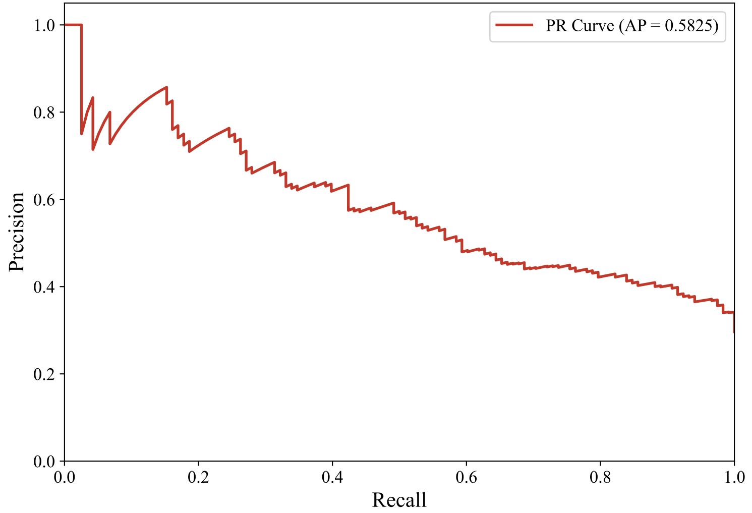
Precision-Recall Curve — DUTCH_MANUAL (upskyy/bge-m3-korean, Random_Forest)
