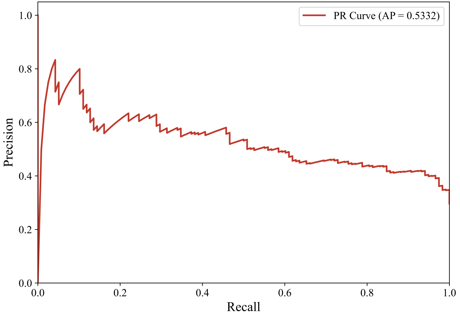
Precision-Recall Curve — DUTCH_MANUAL (xlm-roberta-base, Random_Forest)
