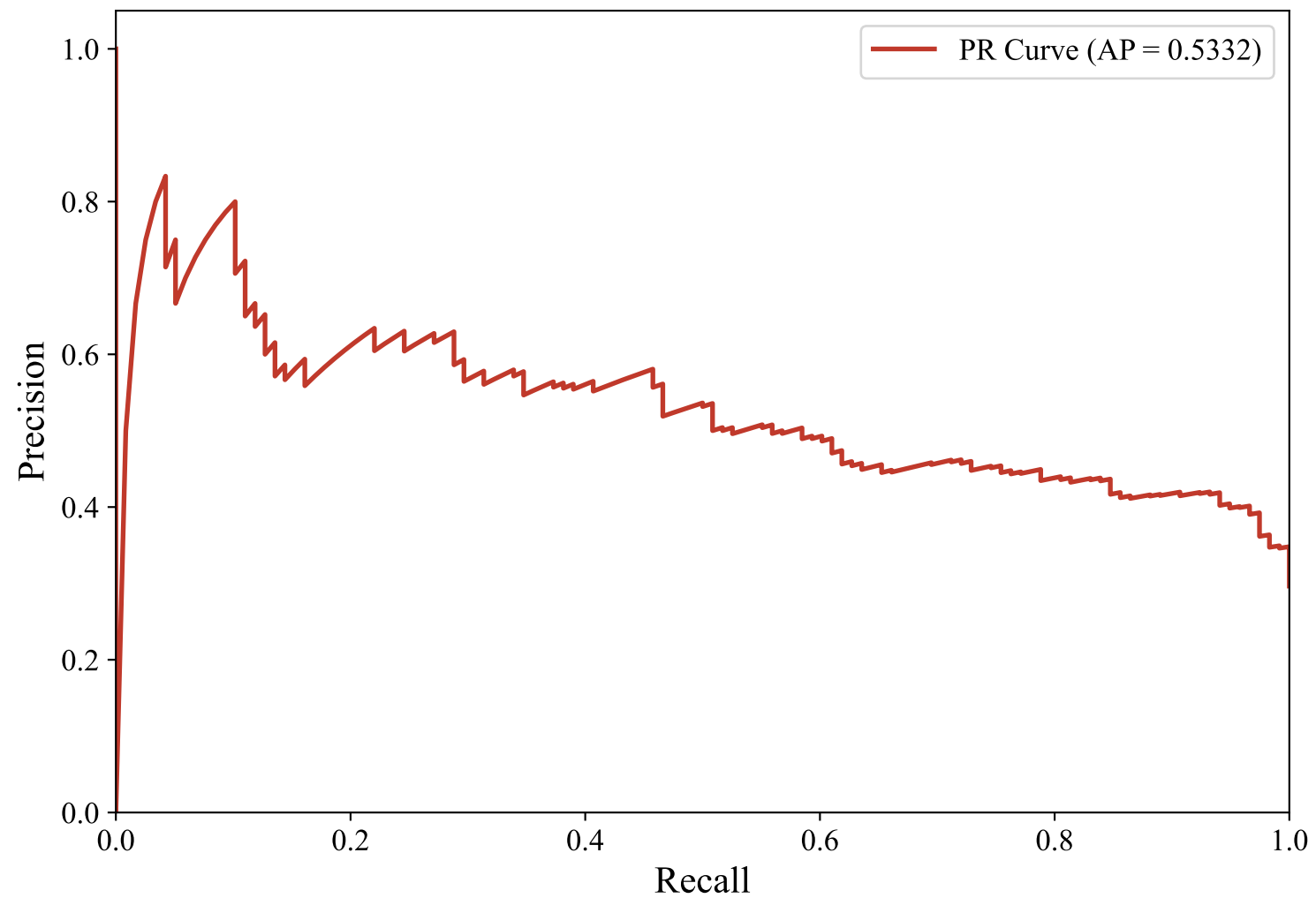
Precision-Recall Curve — DUTCH_MANUAL (xlm-roberta-base, Random_Forest_Optimized)
