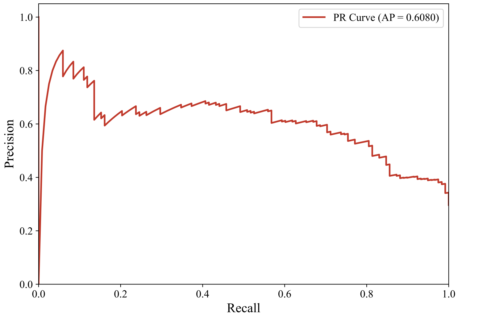
Precision-Recall Curve — DUTCH_MANUAL (xlm-roberta-base, Voting_Ensemble)
