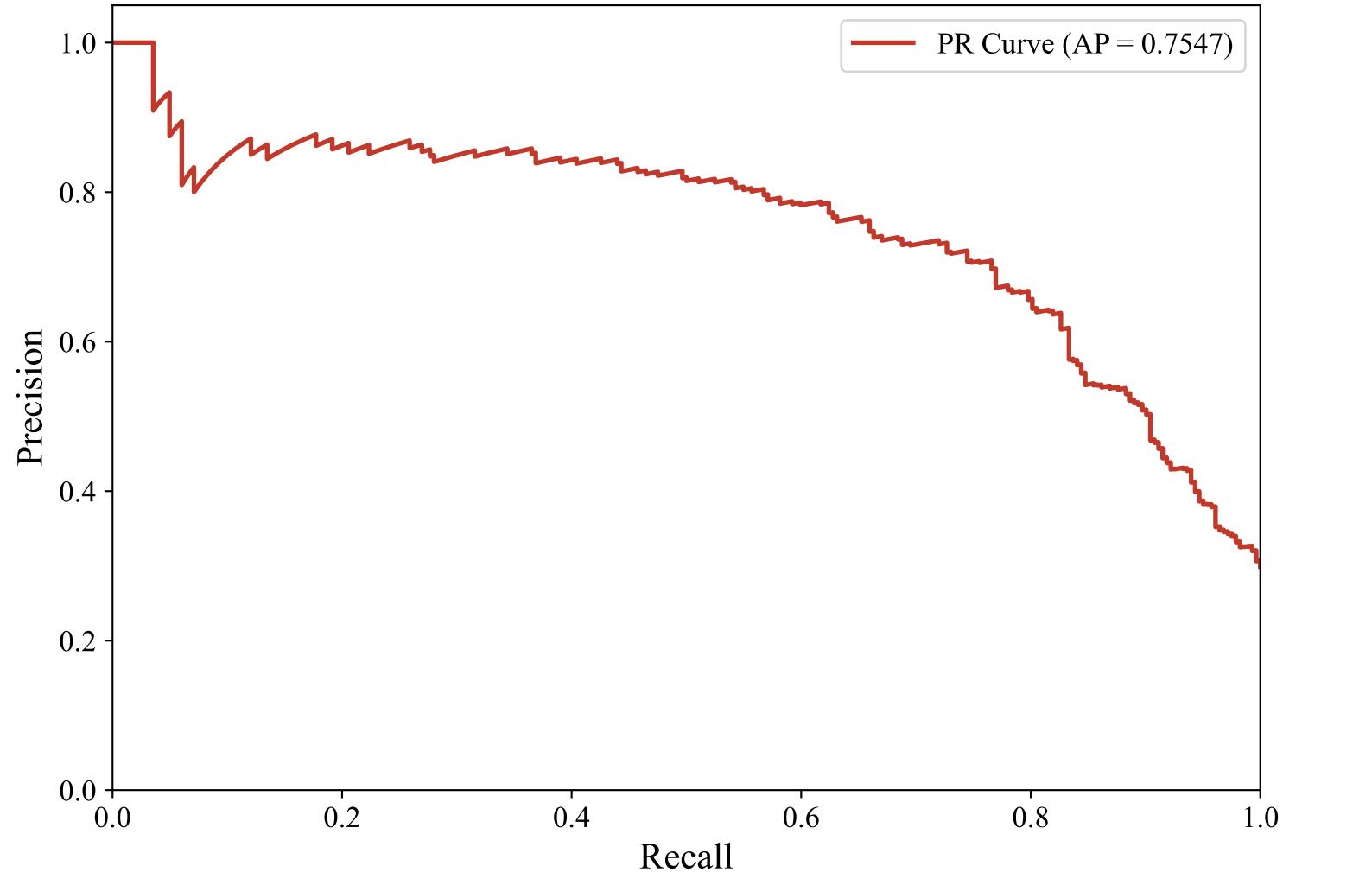
Precision-Recall Curve — ENGLISH_MANUAL (intfloat/multilingual-e5-large-instruct, Voting_Ensemble)
