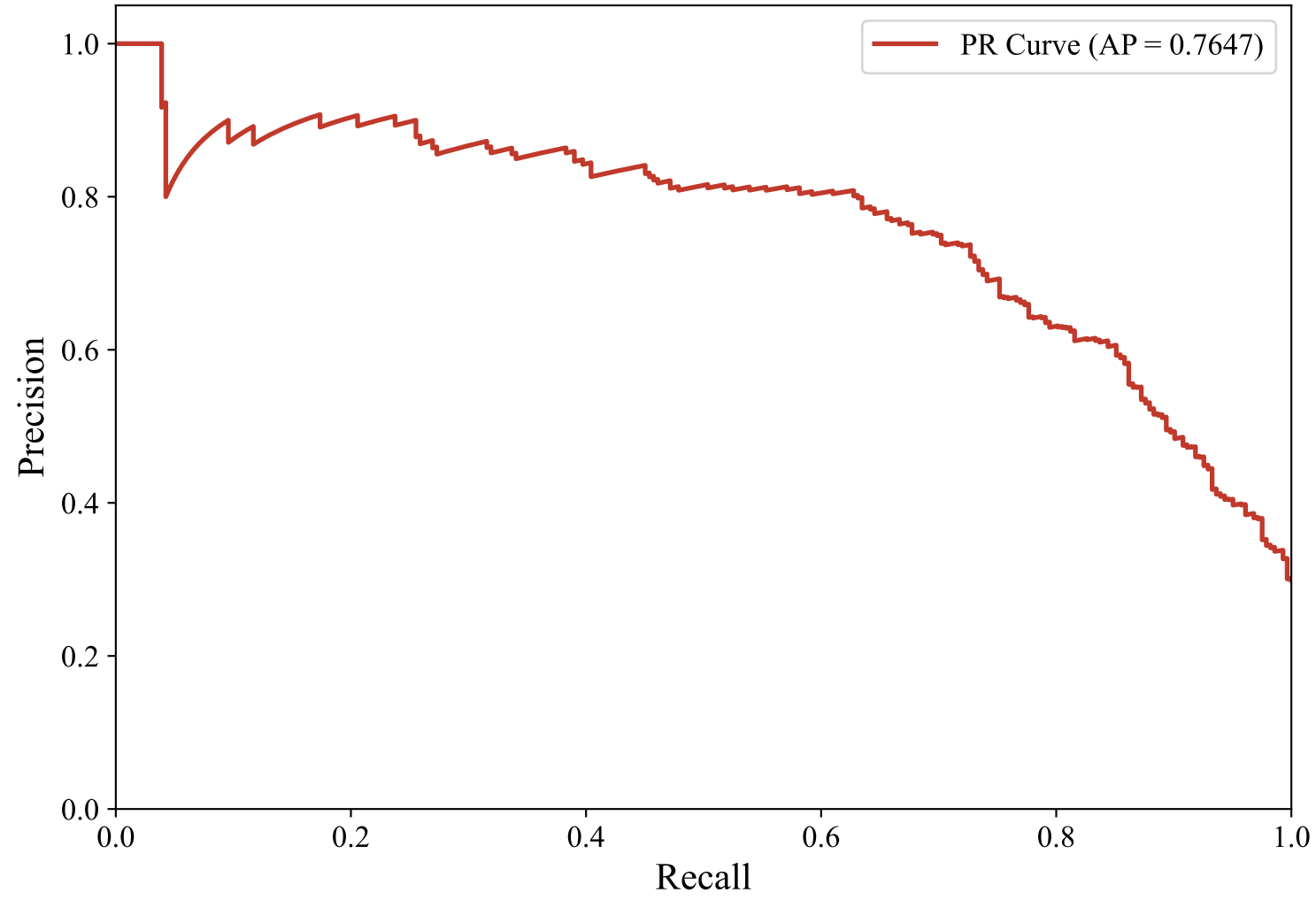
Precision-Recall Curve — ENGLISH_MANUAL (intfloat/multilingual-e5-large-instruct, XGBoost)
