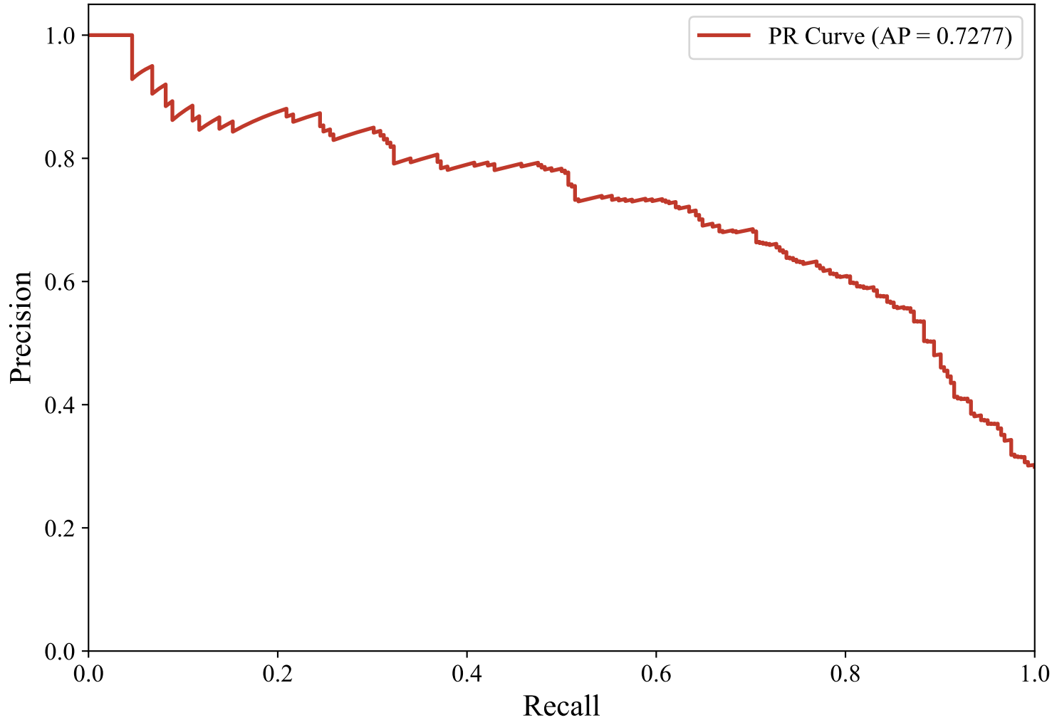
Precision-Recall Curve — ENGLISH_MANUAL (paraphrase-multilingual-MiniLM-L12-v2, LightGBM)
