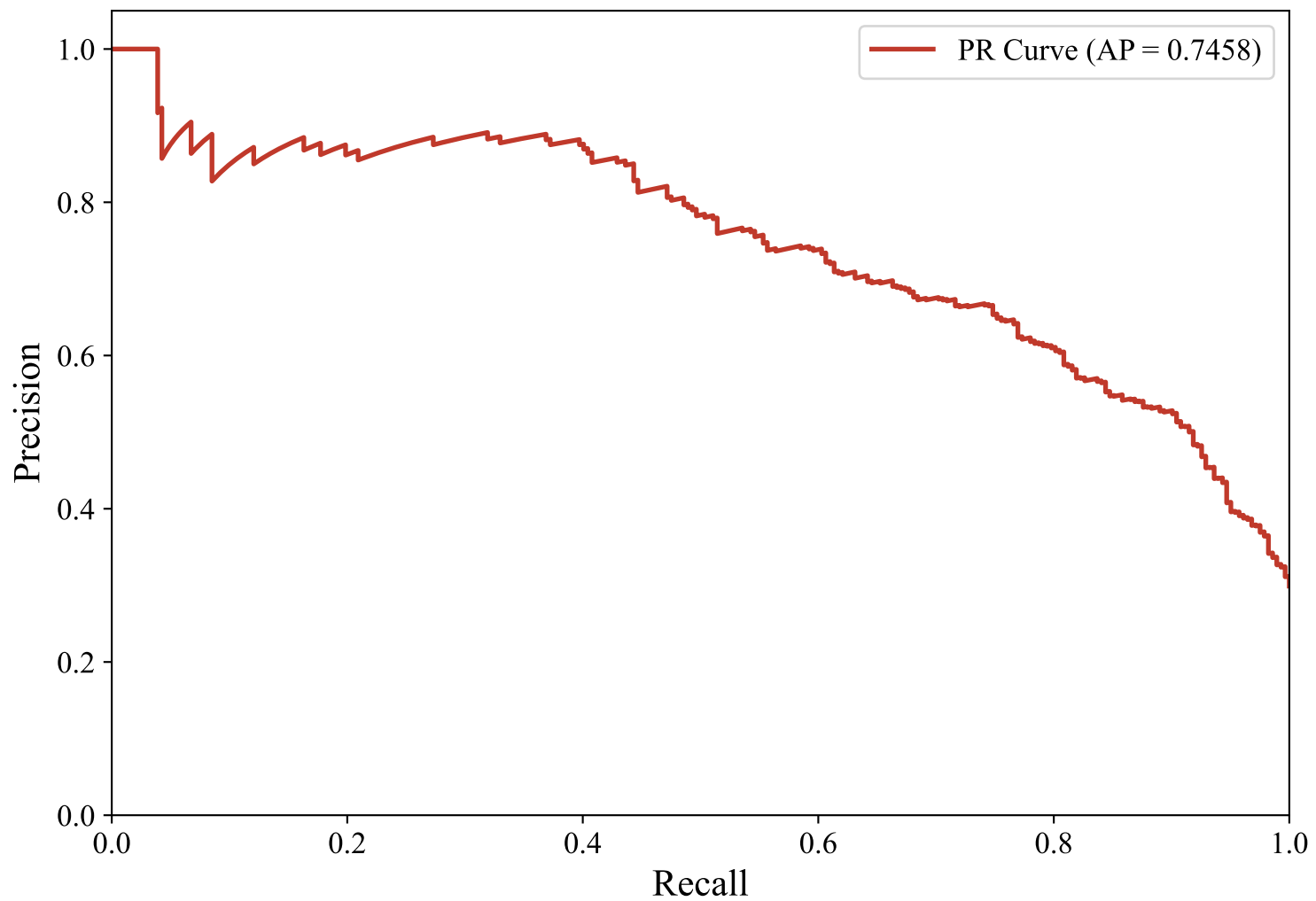
Precision-Recall Curve — ENGLISH_MANUAL (paraphrase-multilingual-mpnet-base-v2, LightGBM_Optimized)
