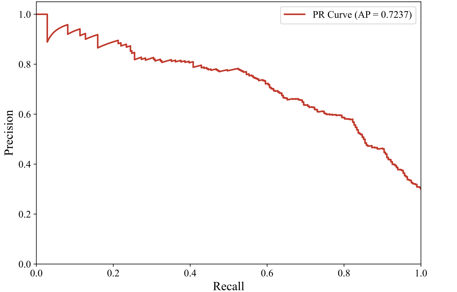
Precision-Recall Curve — ENGLISH_MANUAL (paraphrase-multilingual-mpnet-base-v2, Random_Forest)
