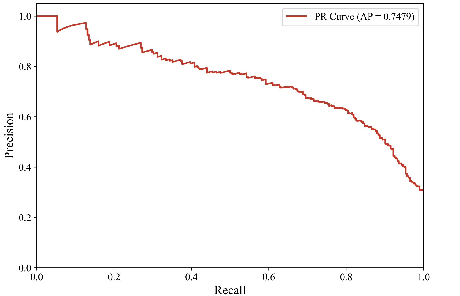
Precision-Recall Curve — ENGLISH_MANUAL (snowflake-arctic-embed-l-v2.0, LightGBM_Optimized)
