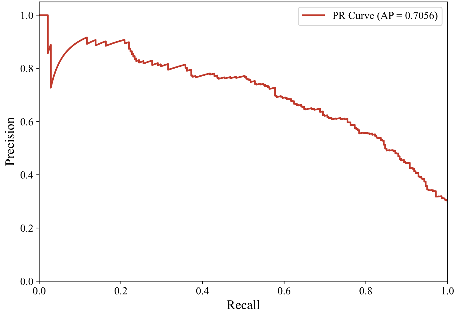
Precision-Recall Curve — ENGLISH_MANUAL (snowflake-arctic-embed-l-v2.0, Random_Forest)
