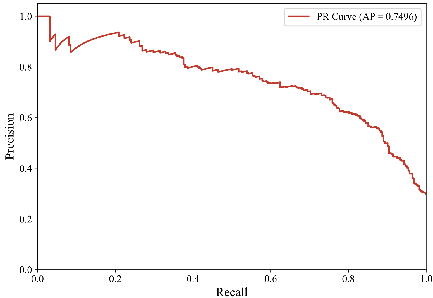
Precision-Recall Curve — ENGLISH_MANUAL (snowflake-arctic-embed-l-v2.0, Voting_Ensemble)
